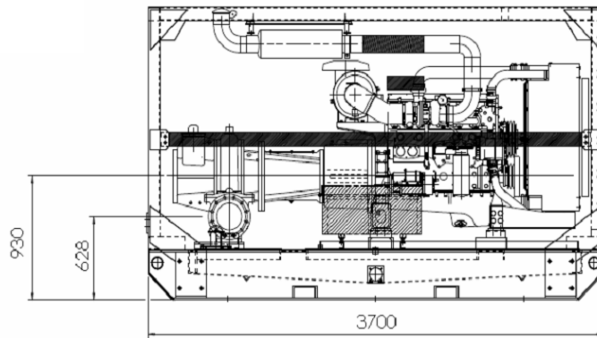
HL225M - Caterpillar C9
