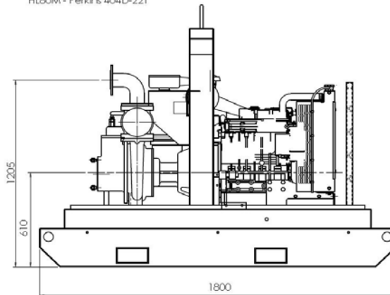
HL80M - Perkins 404D-22T
