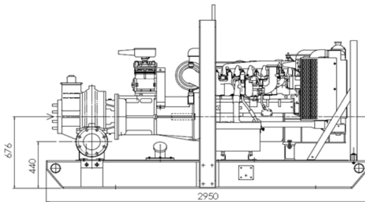
CD180M - Perkins 1106D-E66TA (129)
