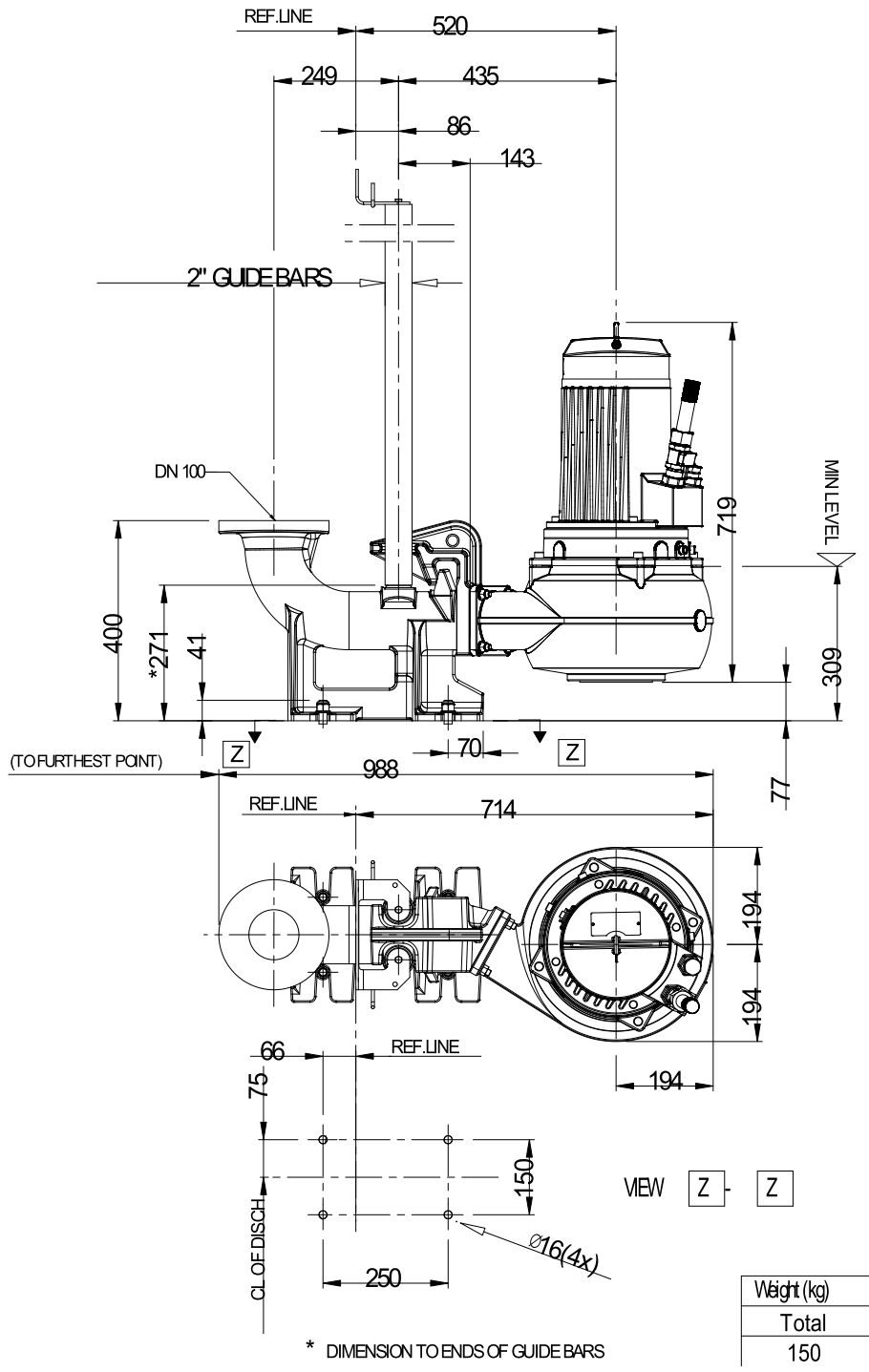
Dimensional dwg DP 8058.280 LT
